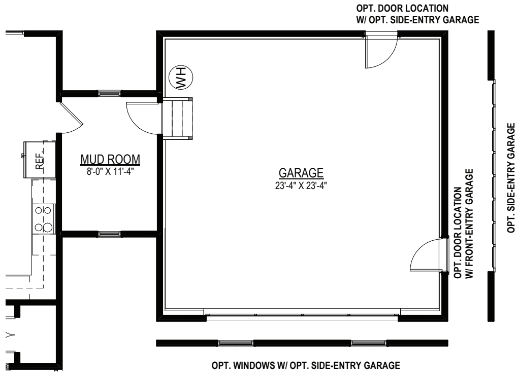
Optional mud room and optional garage
