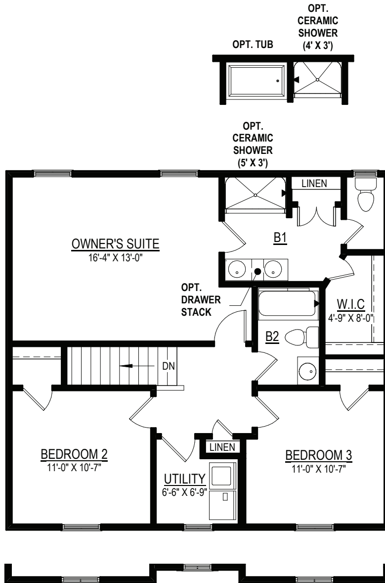
1'-0" SECOND FLOOR BUMP OUT W/ ELEVATION "C"
