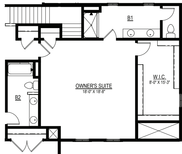
SECOND FLOOR LAYOUT W/ ELEVATION "C"
