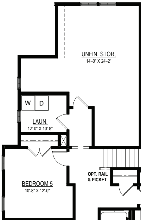
OPT. BEDROOM 5 (IN-LIEU OF LOFT)
