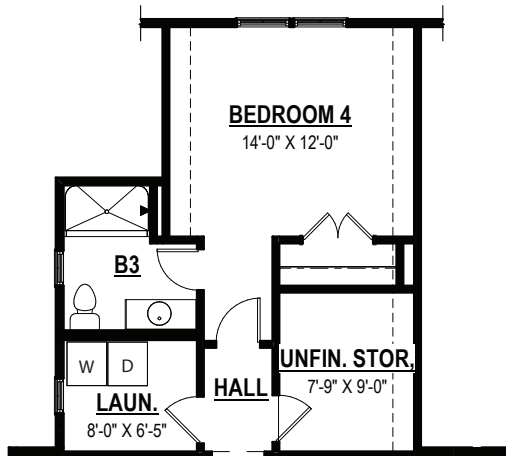
OPT. BEDROOM 4 W/ FULL BATH (IN-LIEU OF UNFIN. STORAGE)
