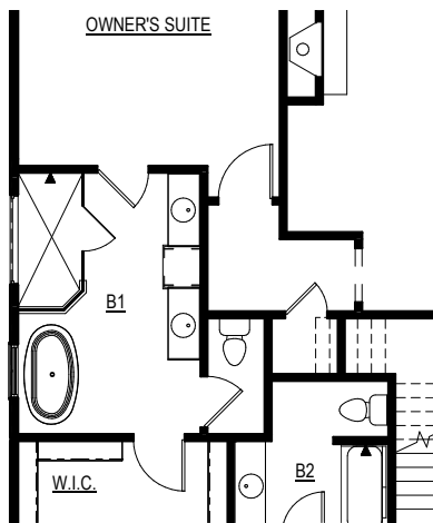
OPT. LUXURY OWNER'S BATH
