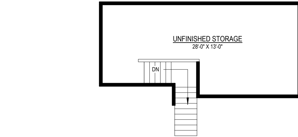
STANDARD SECOND FLOOR
