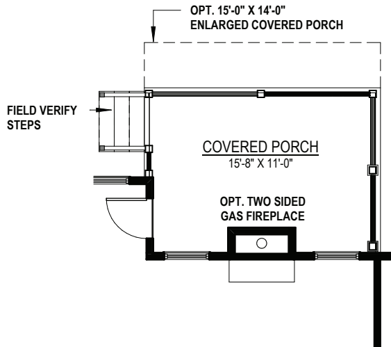
OPT. REAR COVERED PORCH (IN-LIEU OF DECK)
