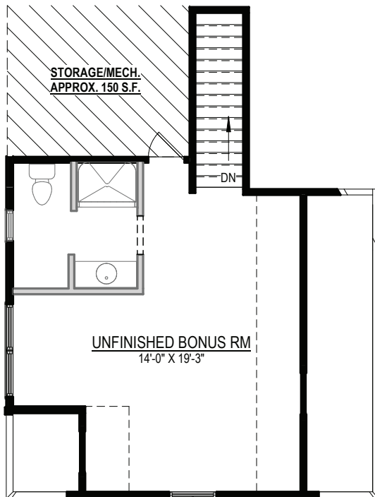
UNFINISHED SECOND FLOOR W/OPT. DOUBLE DORMER & OPT. FULL BATH ROUGH-IN
