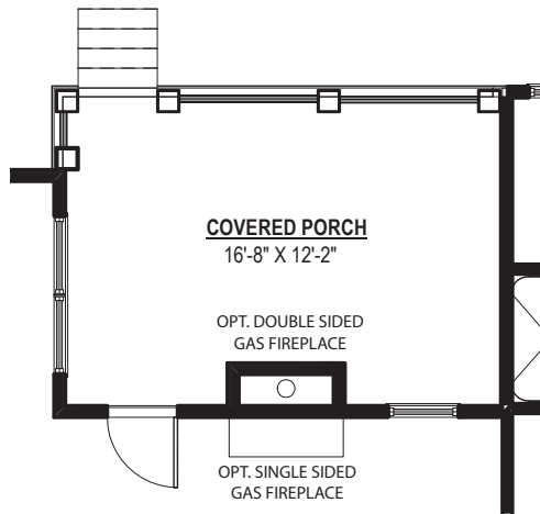
OPT. COVERED PORCH IN LIEU OF FLORIDA ROOM
