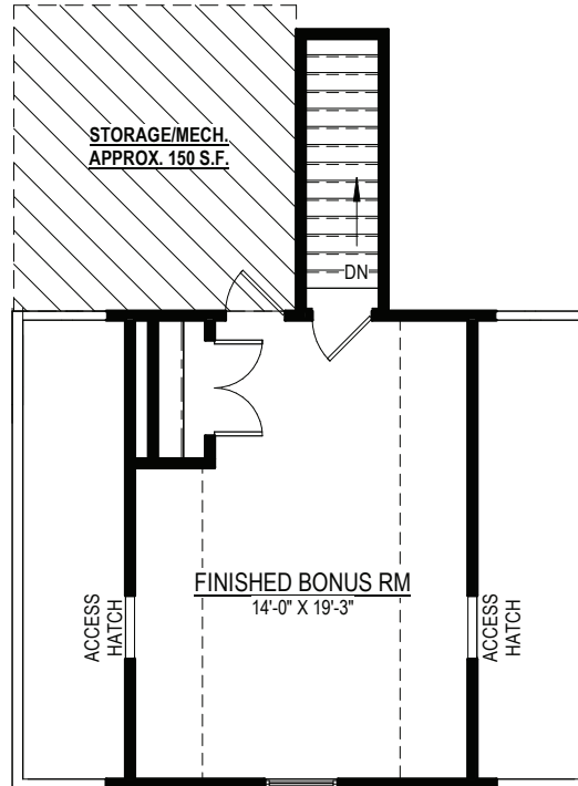
OPTIONAL FINISHED SECOND FLOOR W/CLOSET
