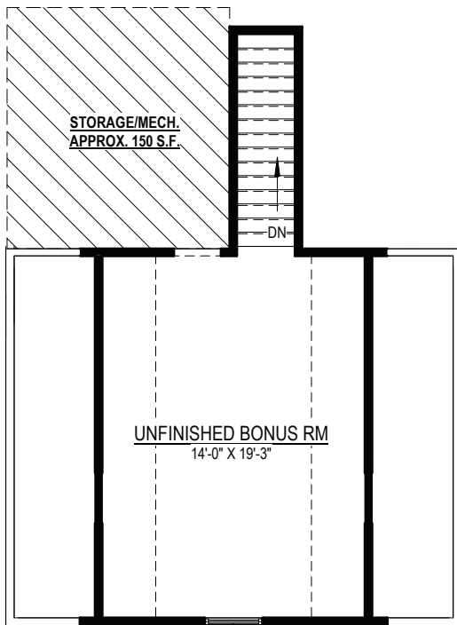
UNFINISHED SECOND FLOOR (STANDARD)
