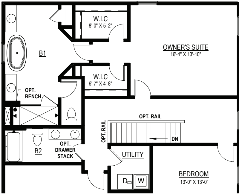
OPT. LUXURY OWNER'S SUITE & BEDROOM IN-LIEU OF LOFT
