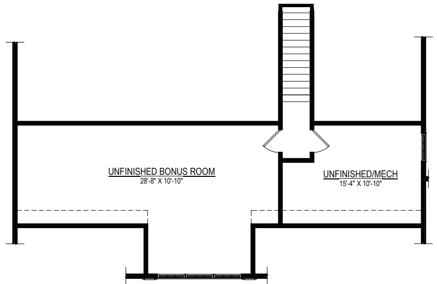
SECOND FLOOR PLAN W/ OPT. UNFINISHED BONUS ROOM
