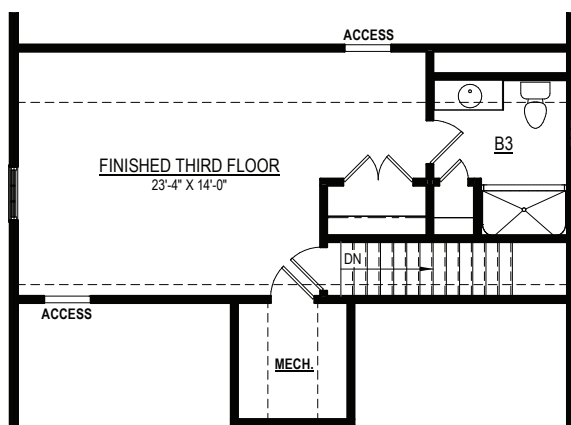
OPT. FINISHED THIRD FLOOR W/ FULL BATH
