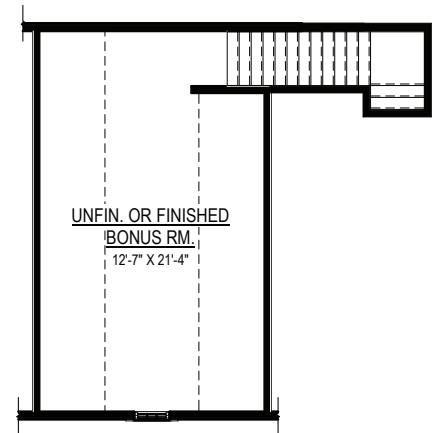
OPT. UNFINISHED OR FINISHED BONUS ROOM OVER GARAGE (W/ GABLE ROOF ONLY)
