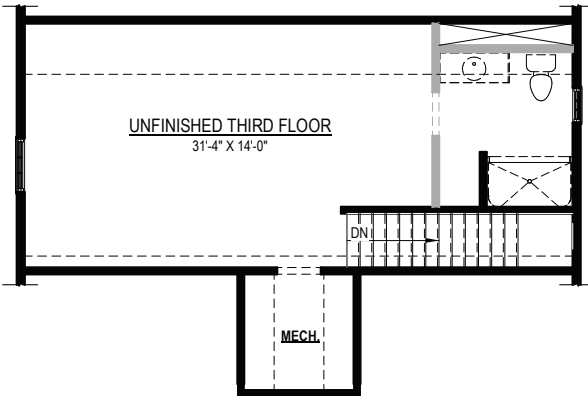
OPT. UNFINISHED THIRD FLOOR W/ OPT. FULL BATH ROUGH-IN
