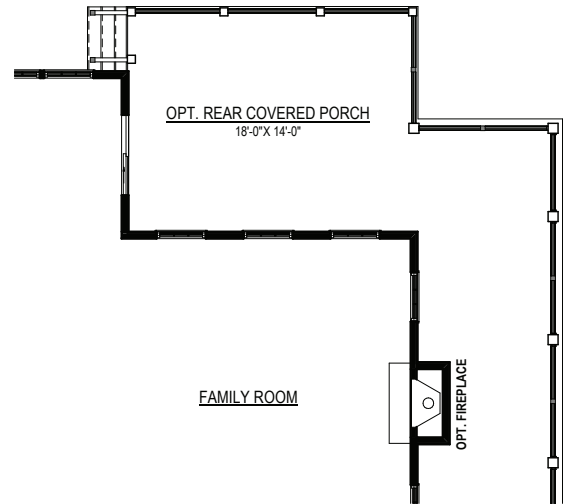
OPT. WRAP AROUND PORCH
