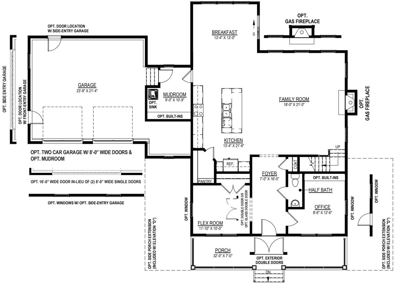
FIRST FLOOR PLAN (SHOWN W/ OPTIONAL MUD ROOM AND GARAGE)
