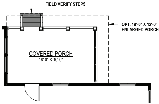
OPT. COVERED PORCH (IN-LIEU OF DECK)
