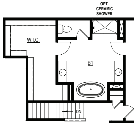
OPT. FREESTANDING TUB IN OWNER'S BATH
