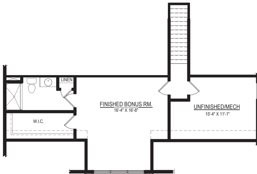
SECOND FLOOR PLAN W/ OPT. FINISHED BONUS ROOM & OPT. FULL BATH
