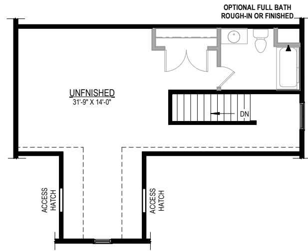
OPT. UNFINISHED OR FINISHED THIRD FLOOR
